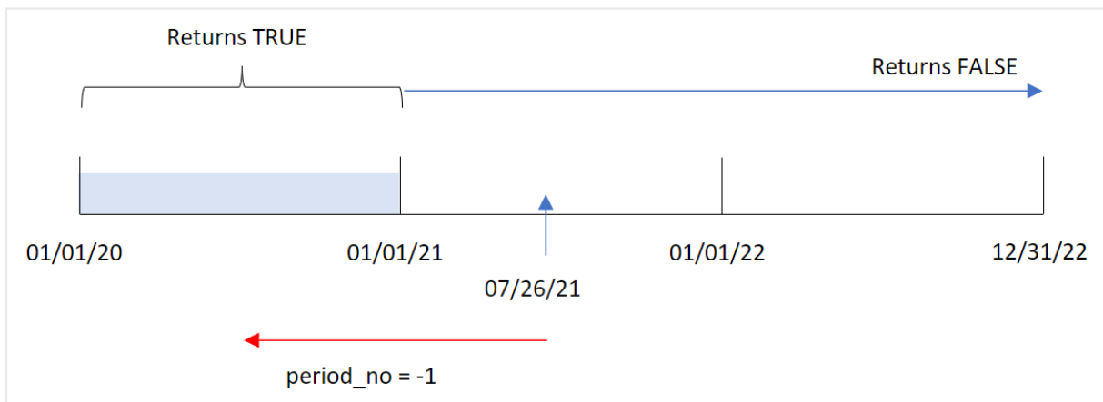
Diagram of inyear() function's range with the period_no argument set to -1
