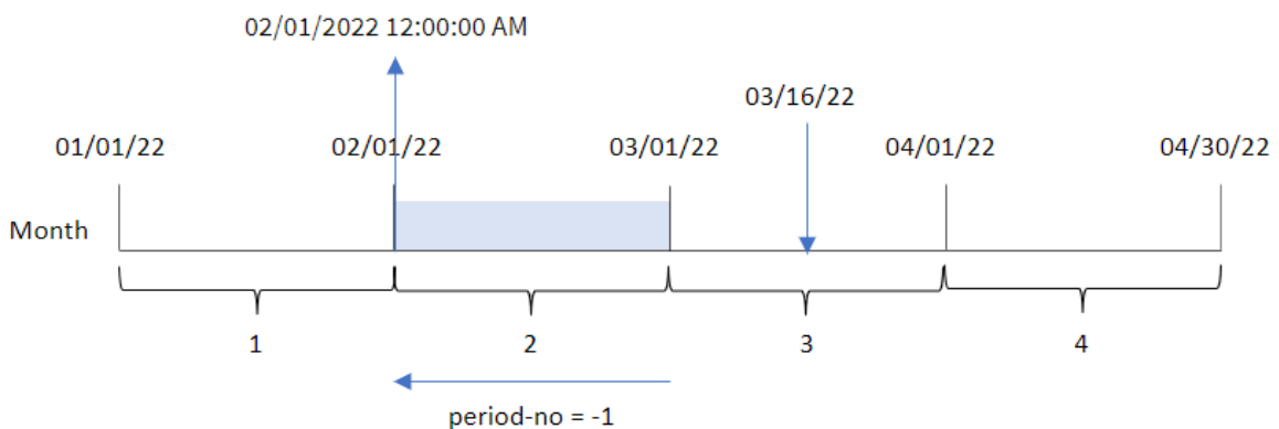
Diagram of monthstart() function, period_no example
