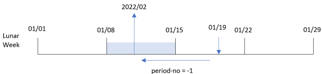
Diagram of lunarweekname() function, period_no example
