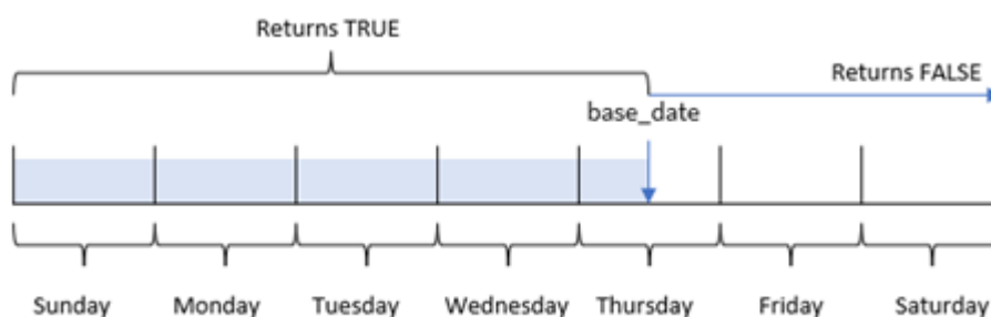
Diagram of inweektodate function
