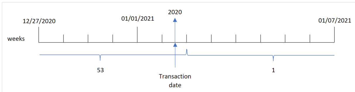
Diagram of weekyear() function's range when using unbroken weeks
