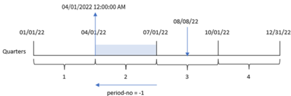
Diagram of quarterstart() function, period_no example
