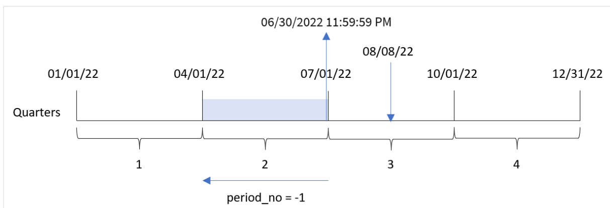
Diagram of the quarterend() function with a period_no of -1
