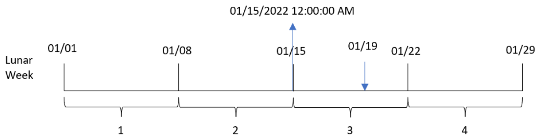
Diagram of lunarweekstart() function, example with no additional arguments
