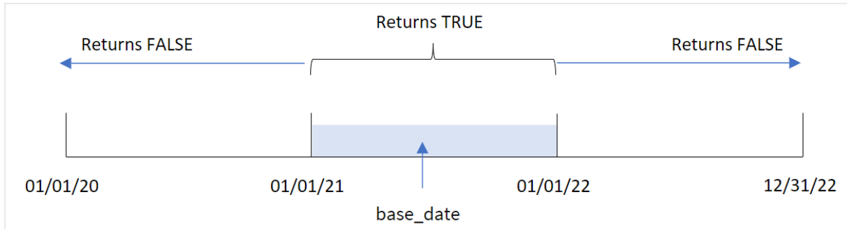
Diagram of inyear() function's range
