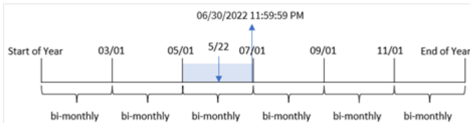
Diagram of monthsend function with bi-monthly segments.
