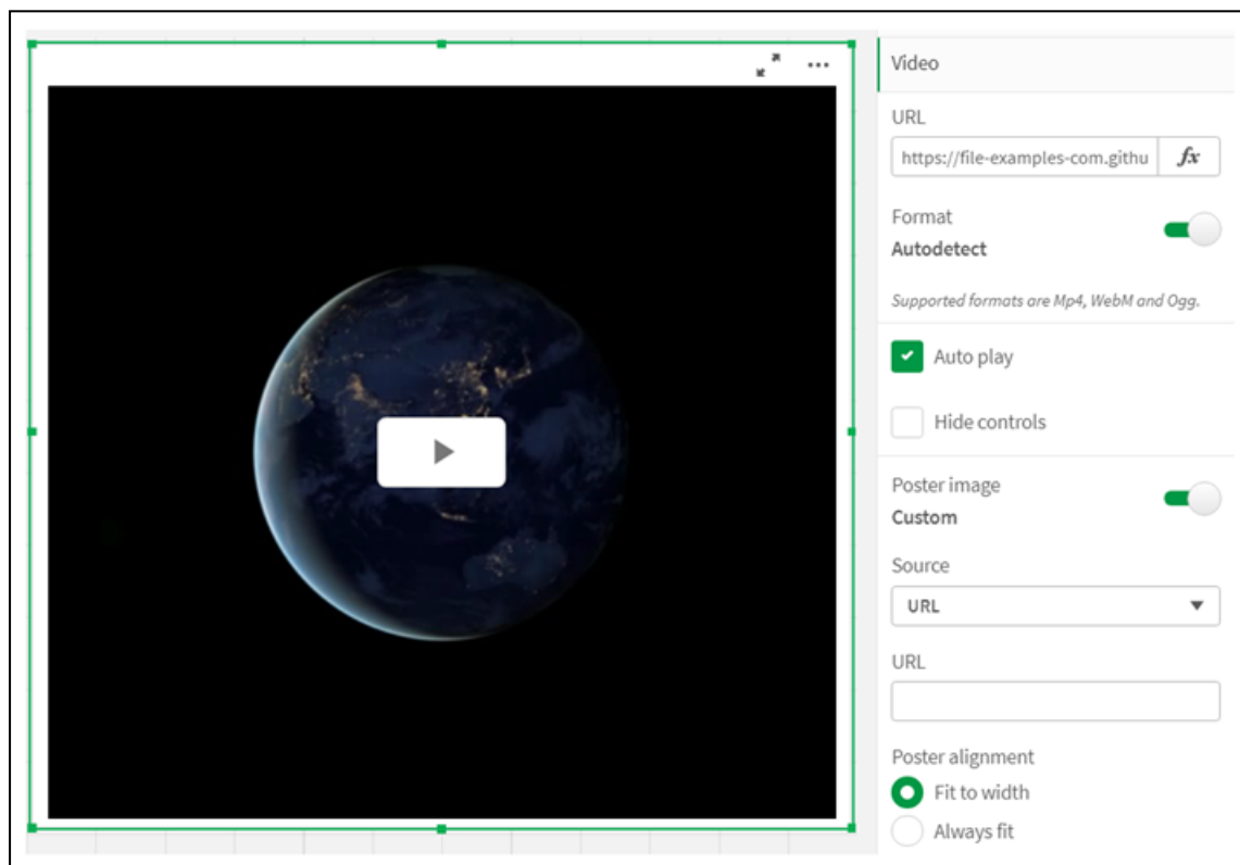
Video-Player
